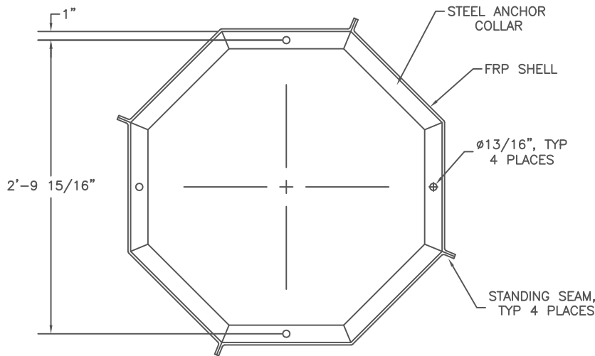
2 ANCHOR COLLAR PLAN S1
