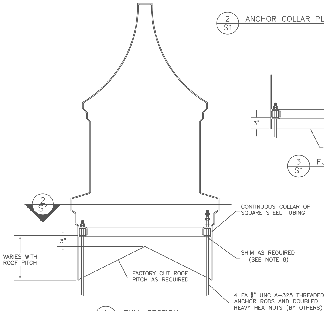
1 FULL SECTION S1
