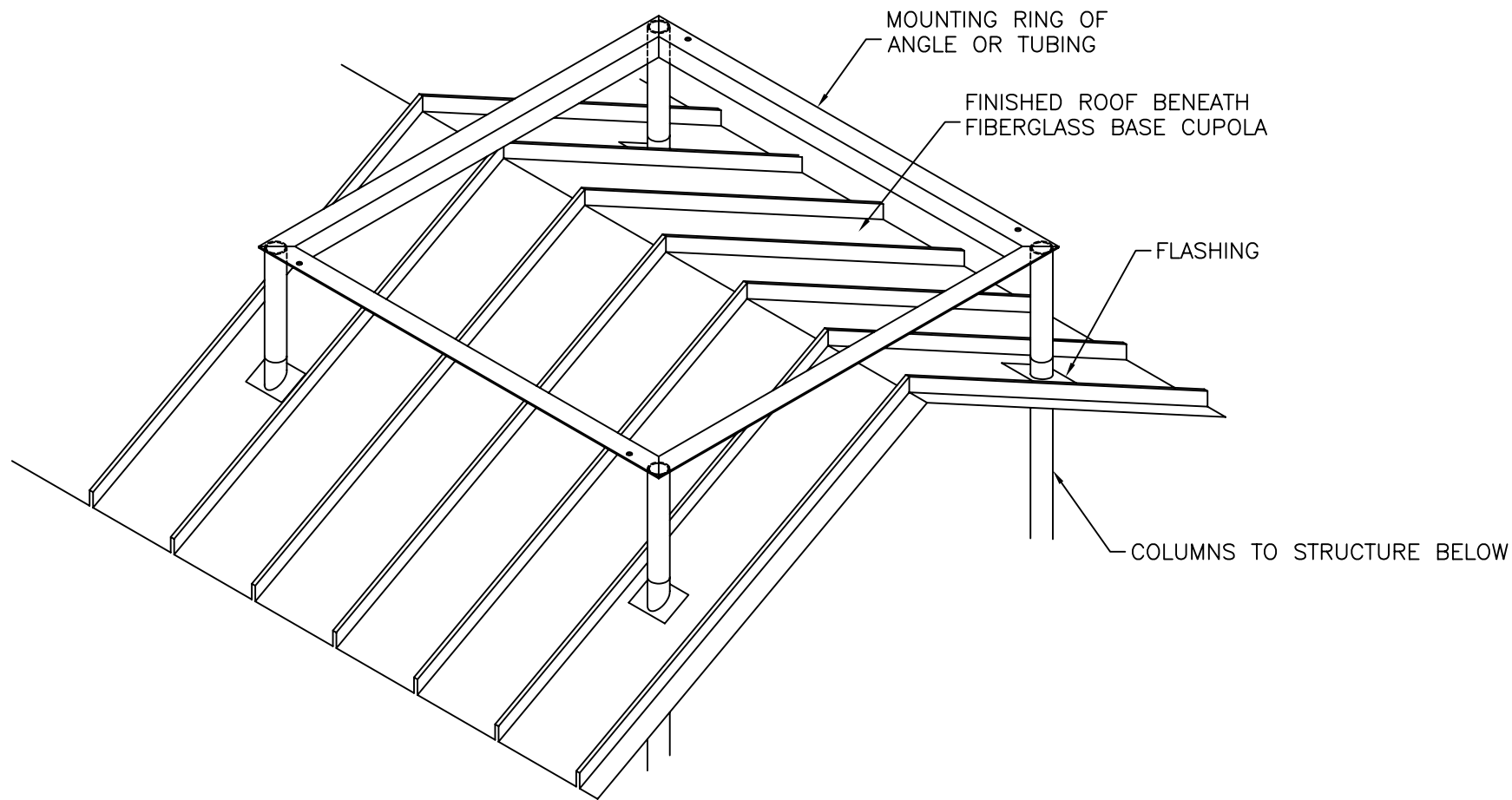
ROOF PREPARED TO RECEIVE CUPOLA
