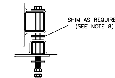
3 S1 BOLTING DETAIL
