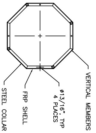
2 TOP OF CU-704 S2
