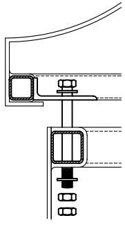
3 BOLTING DETAIL S1
