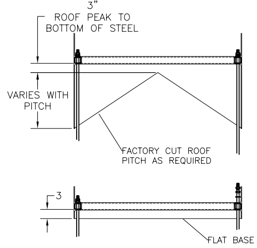
4 BASE DETAILS S1
