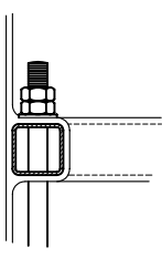
2 ANCHOR DETAIL S1
