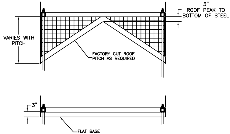
4 S1 BASE DETAILS
