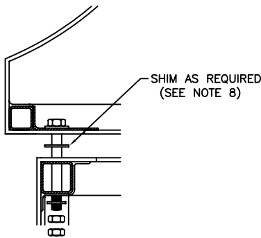
3 S1 BOLTING DETAIL
