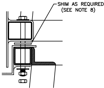
4 BOLTING DETAIL S1
