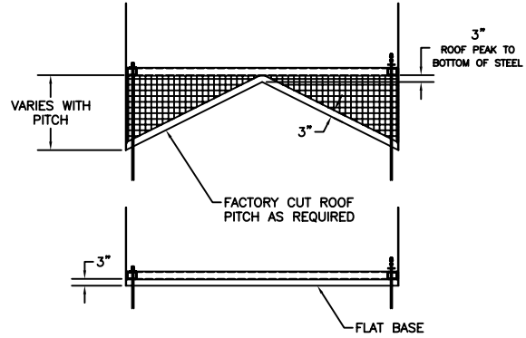
5 BASE DETAILS S1
