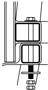
3 BOLTING DETAIL S1
