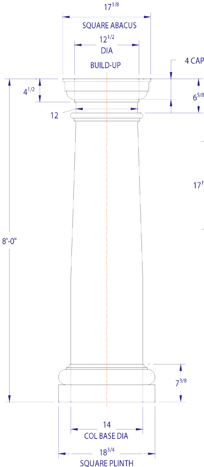
14" DIAMETER COLUMN - TUSCAN
